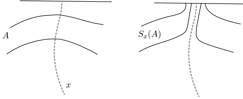
Figure 2: The effect of the arc surgery operator S_x .
