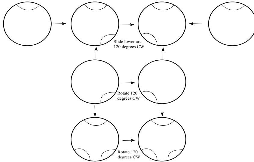
Figure 1: Calculation in the localised category representing the total space, showing the the generator of the fundamental group of the fibre is trivial in the total space. The unlabelled arrows in this diagram are all the evident inclusions of arc systems.
